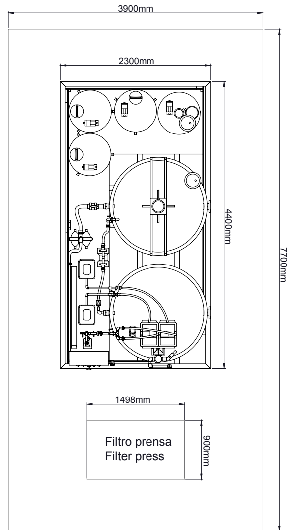
Dimensions and required installation area
